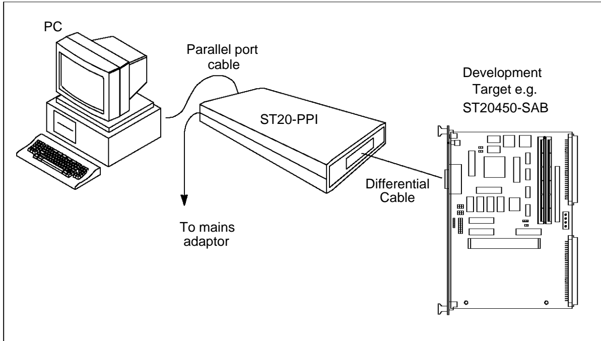
Figure 2.1 ST20-PP1 connections
